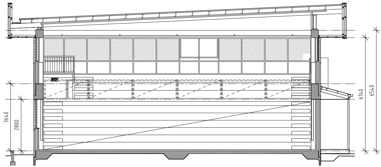
Theatre - Elevation
