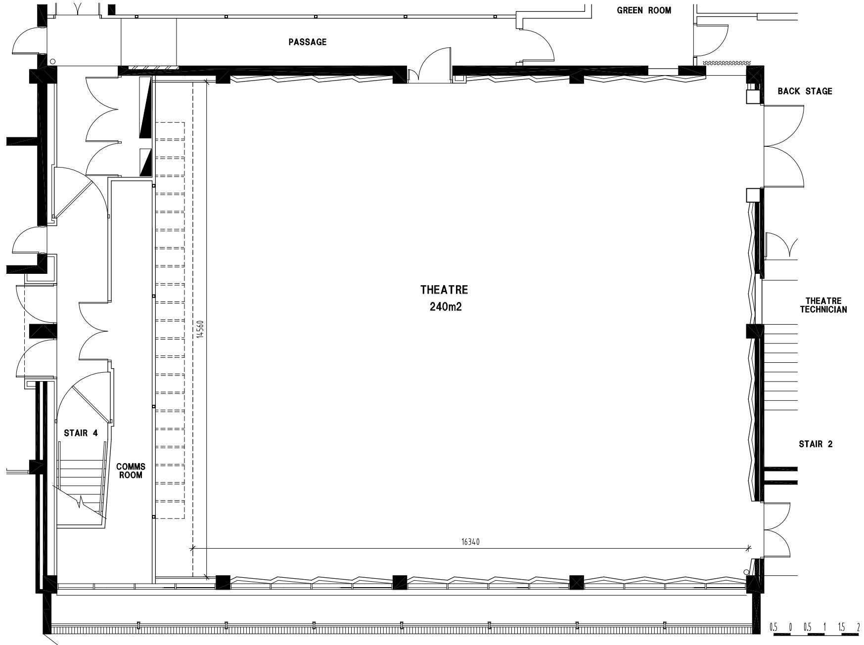
Theatre Plan
